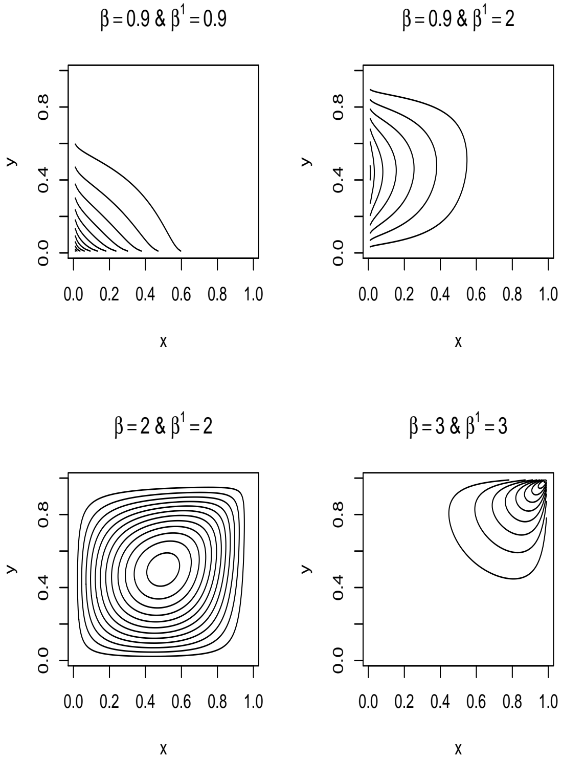
FIGURE 1. Plots of the pdf of (1) for \gamma = 5 , \gamma' = 5 , \alpha = 2 , u = 0.5 , v = 0.5 and selected values of (\beta, \beta') .
