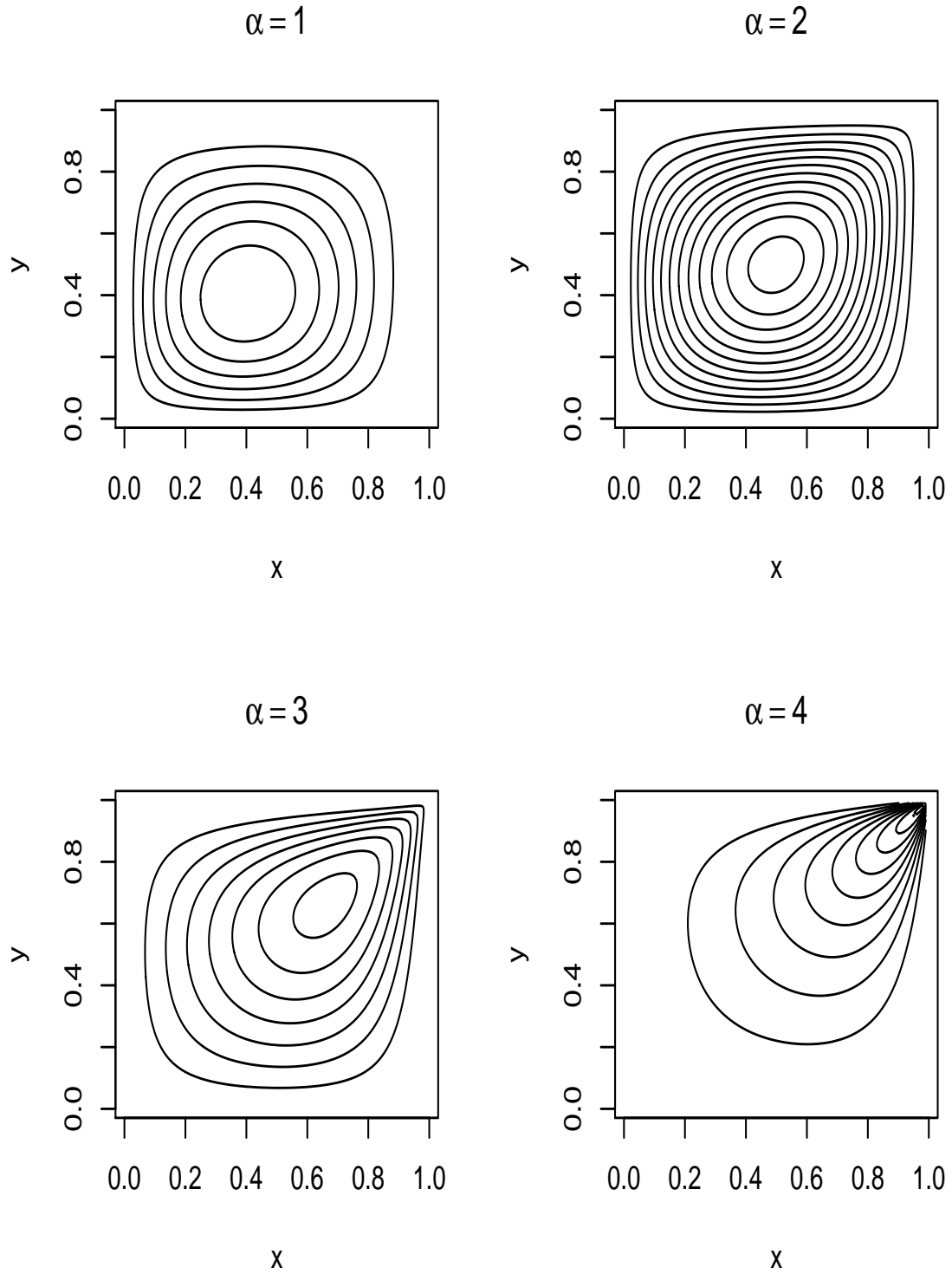
FIGURE 2. Plots of the pdf of (1) for \beta = 2 , \beta' = 2 , \gamma = 5 , \gamma' = 5 , u = 0.5 , v = 0.5 and selected values of \alpha .
