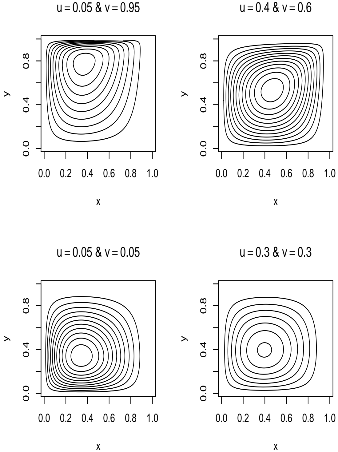
FIGURE 3. Plots of the pdf of (1) for \beta = 2 , \beta' = 2 , \gamma = 5 , \gamma' = 5 , \alpha = 2 and selected values of (u, v) .
